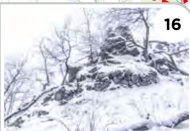
RAGÁČ NNR Slag cone with lava flow, stone run
